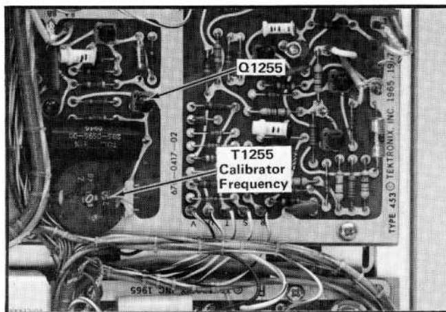
Fig. 5-6. Location of calibrator adjustments.
