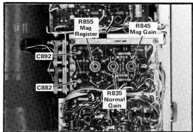
Fig. 5-14. Location of Horizontal Amplifier adjustments (B Sweep board).
