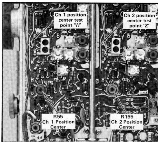
Fig. 5-8. Location of position center test points and adjustments (Vertical Preamp board).
