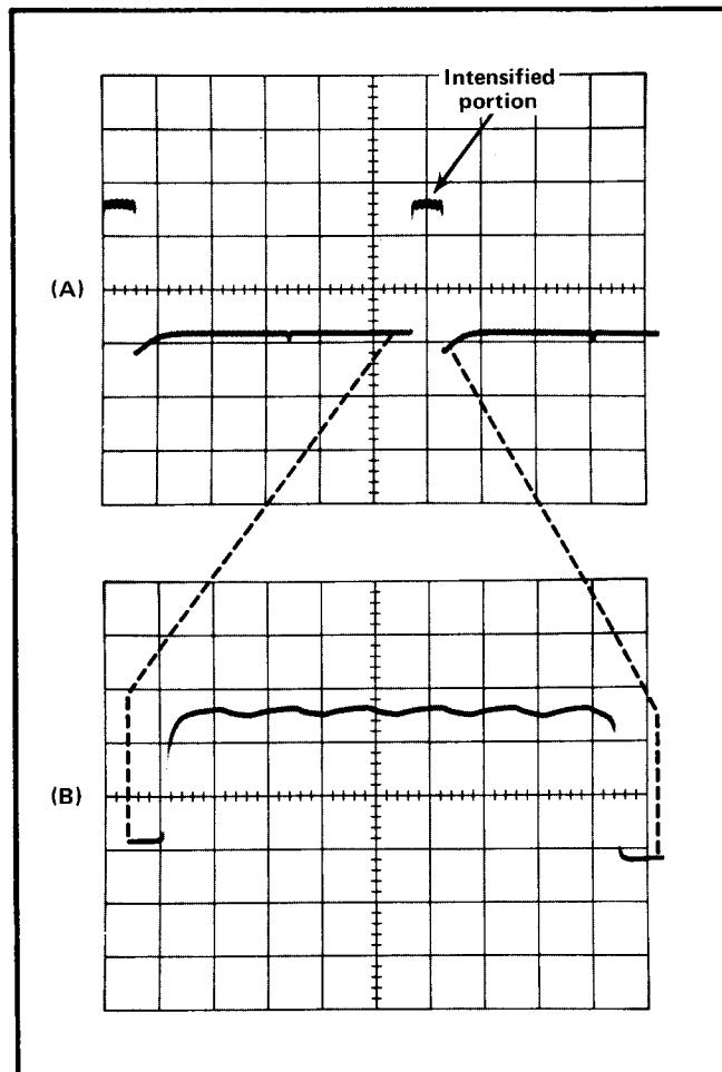
Fig. 2-13. (A) A INTEN DURING B display (A TIME/DIV, .5 ms; B TIME/DIV, 50 \mu s), (B) B (DELAYED SWEEP) display.
