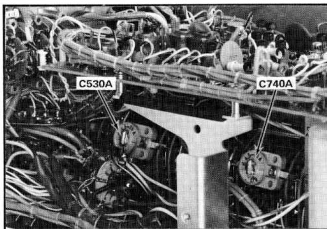
Fig. 5-15. Location of one-microsecond timing adjustments (behind swing-out side panel).
