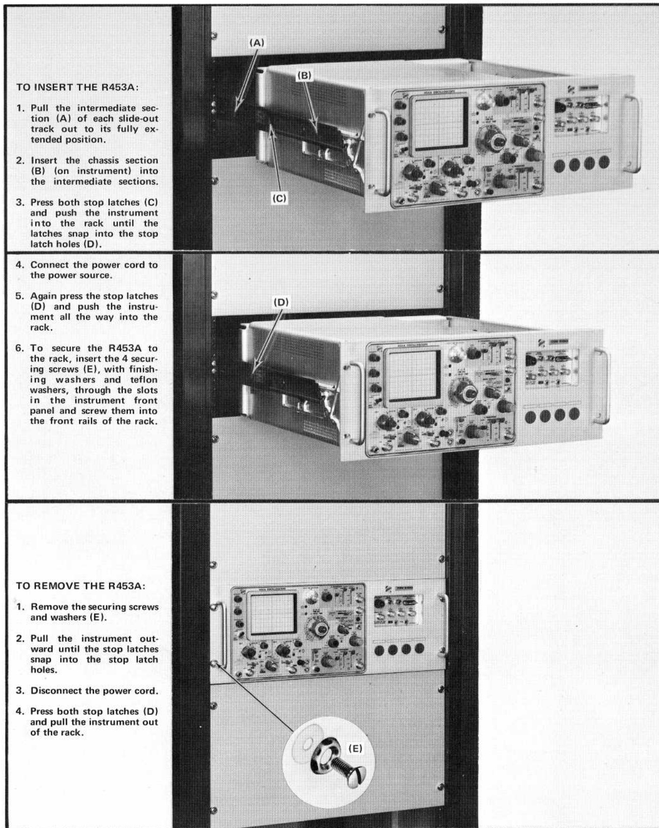
Fig. 6-8. Procedure for inserting or removing the instrument after the slide-out tracks have been installed.
