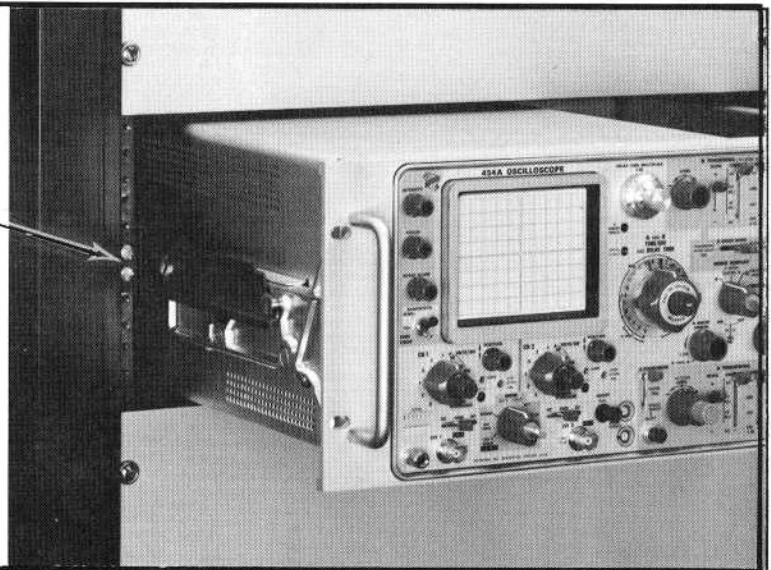
Fig. 6-9. Alignment adjustments for correct operation.
