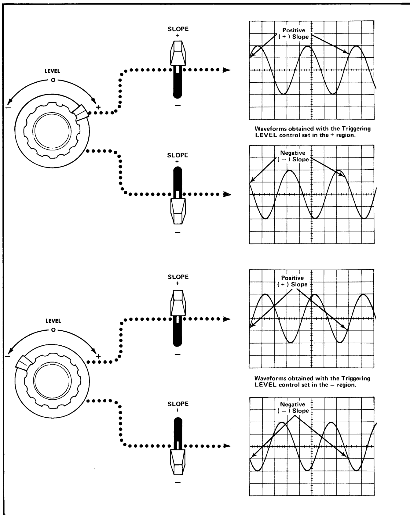
Fig. 2-9. Effects of Triggerring LEVEL control and SLOPE switch.
