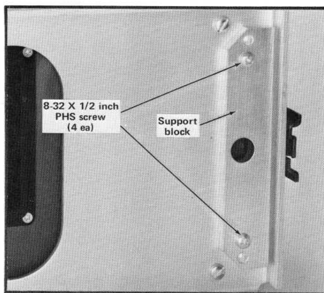
Fig. 6-7. Installing the support block on the instrument.
