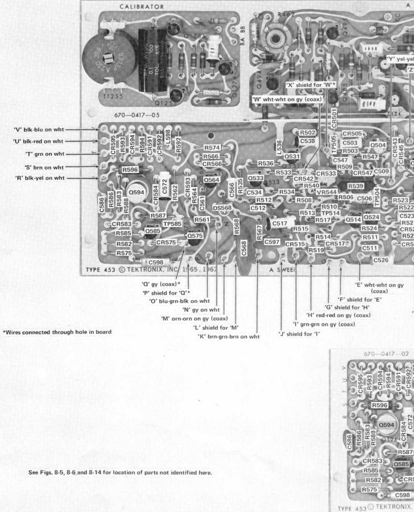
Fig. 8-7. P/O A3. Partial A Sweep circuit board
