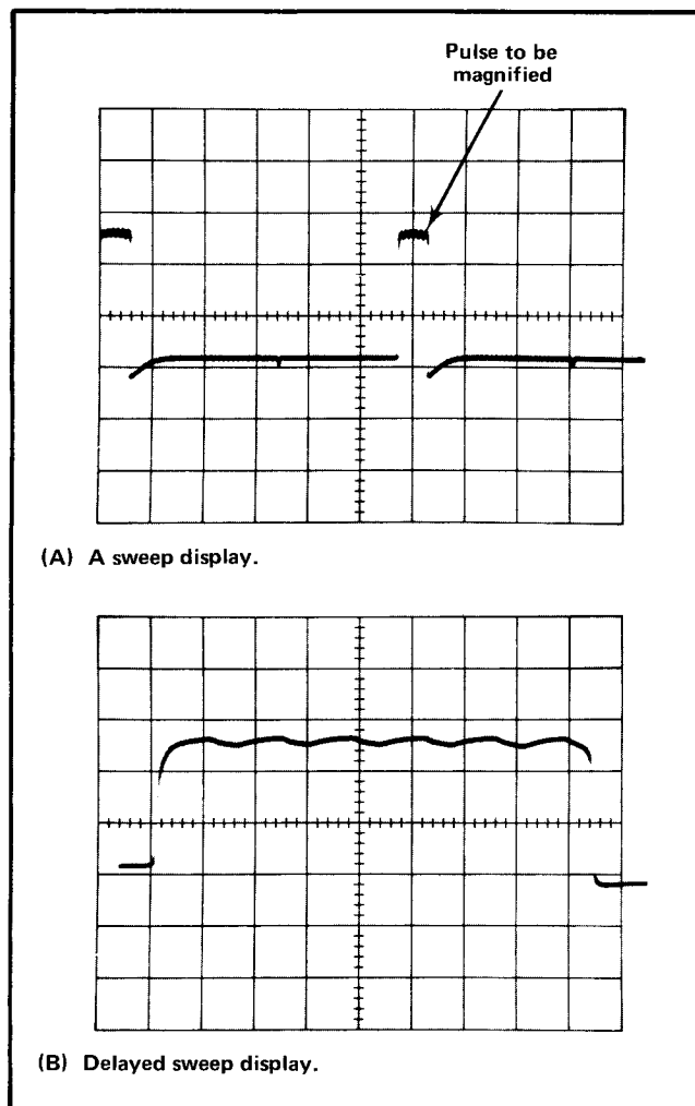
Fig. 2-23. Using delayed sweep for sweep magnification.
